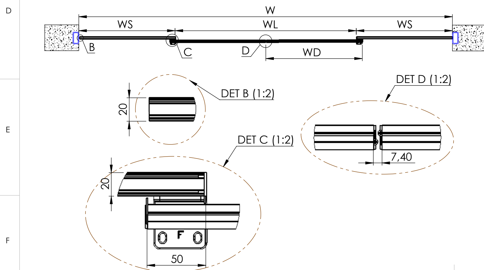
Horizontal section:
