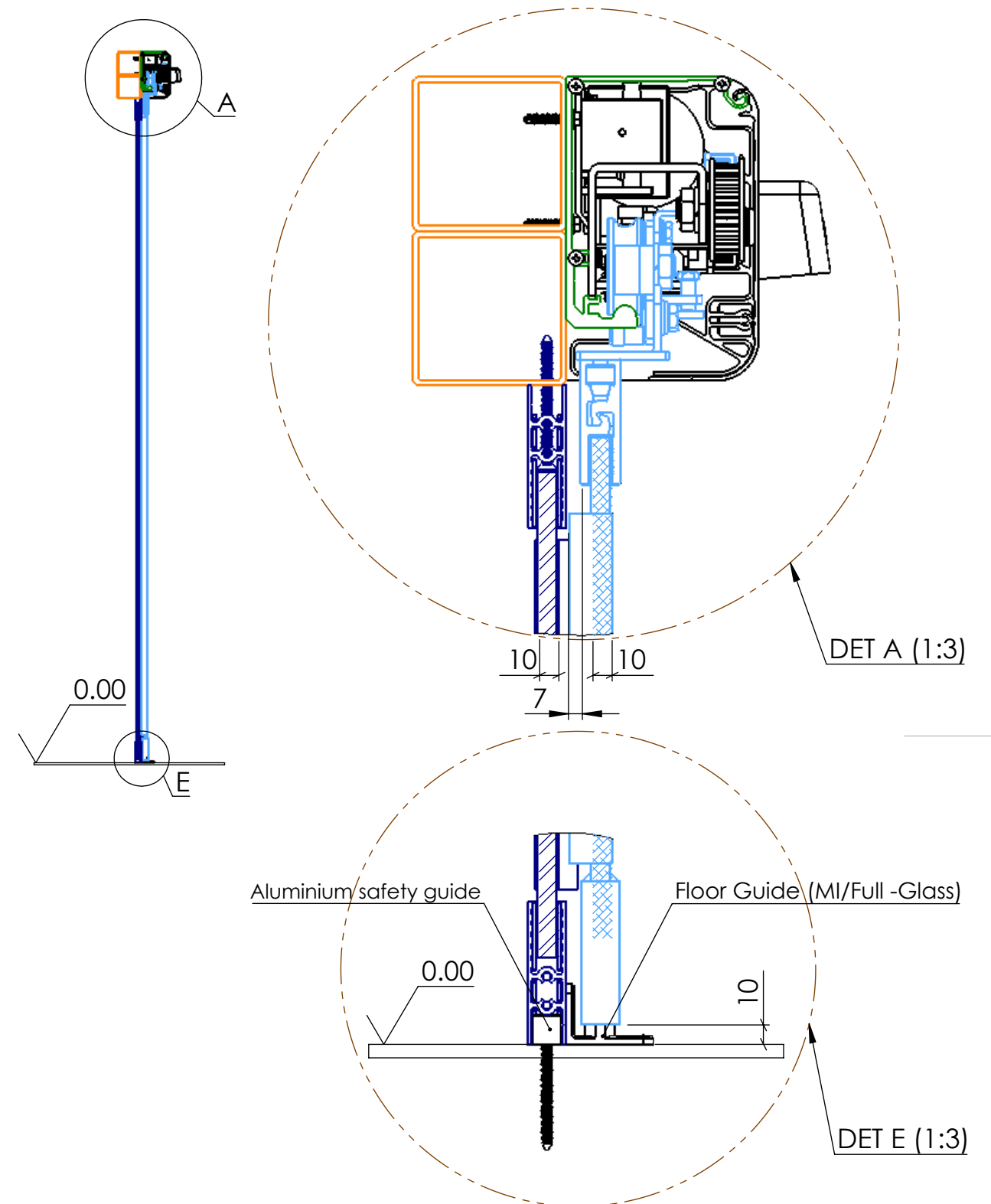
Vertical section: Beam profile
