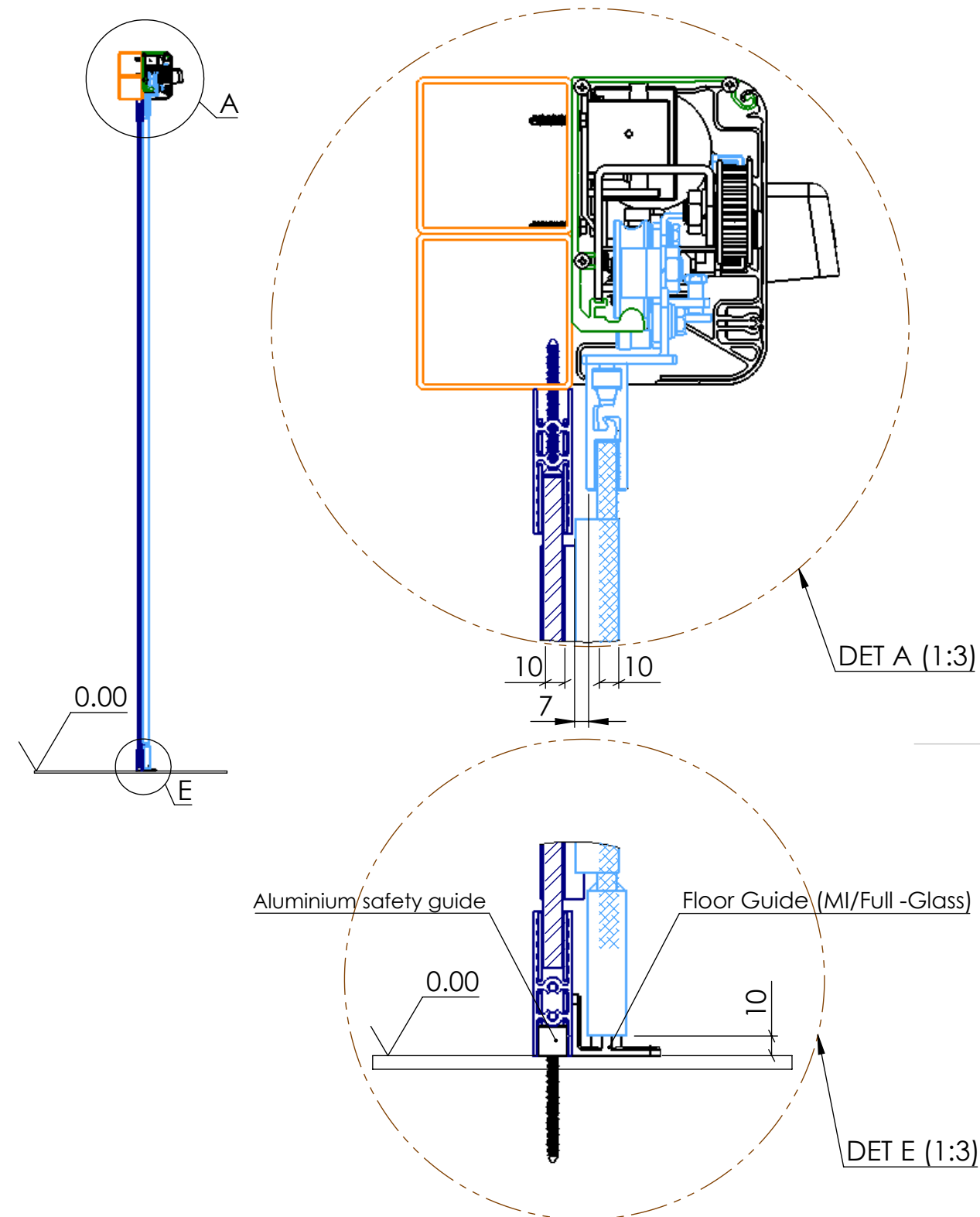
Vertical section: Beam profile
