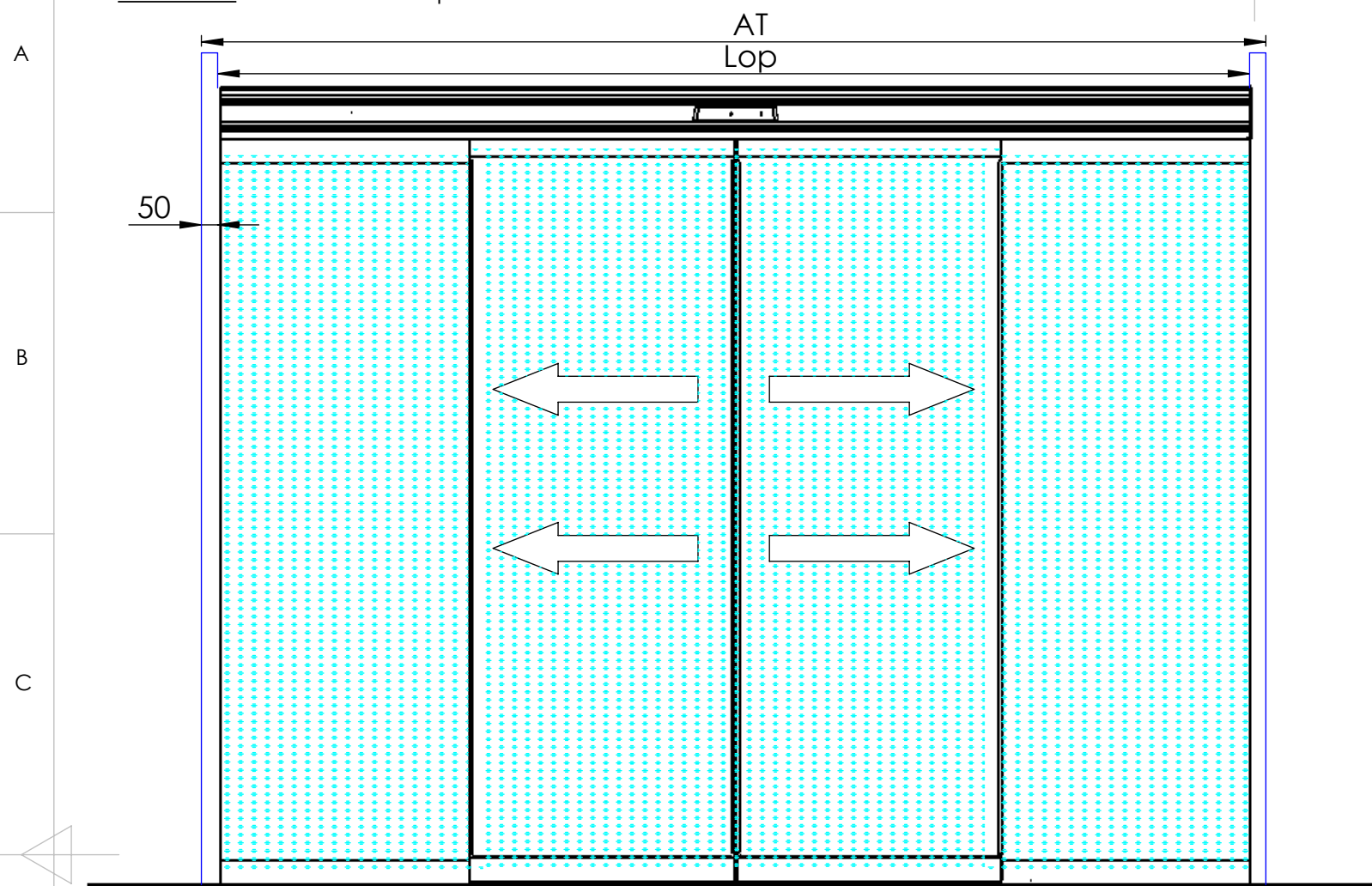
Elevation: View from the operator side
