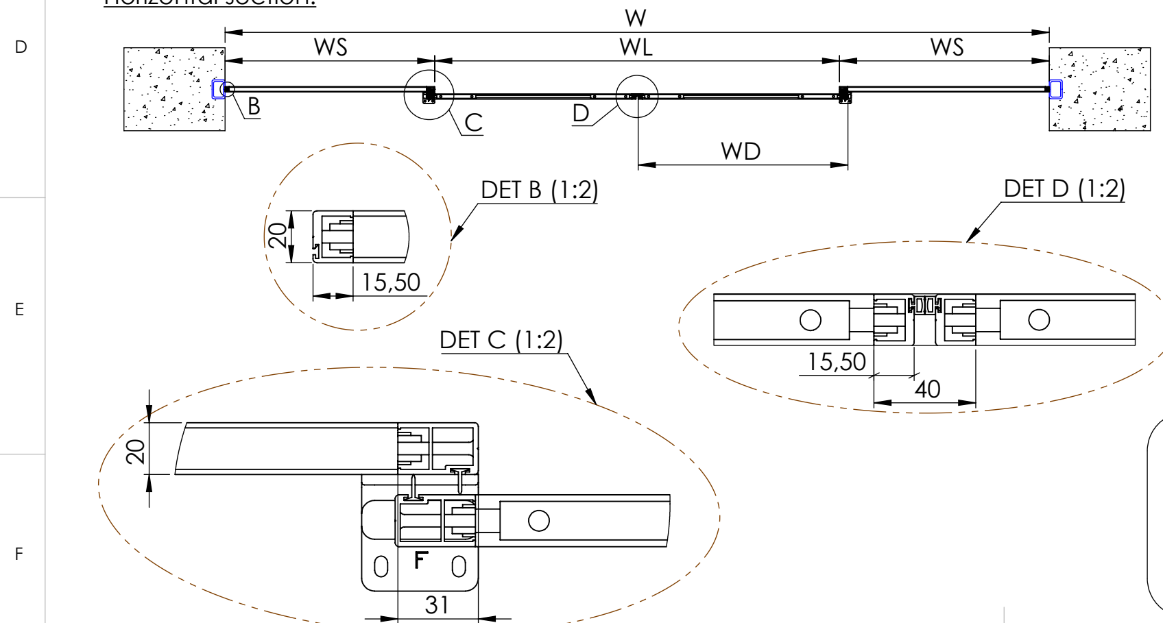
Horizontal section:
