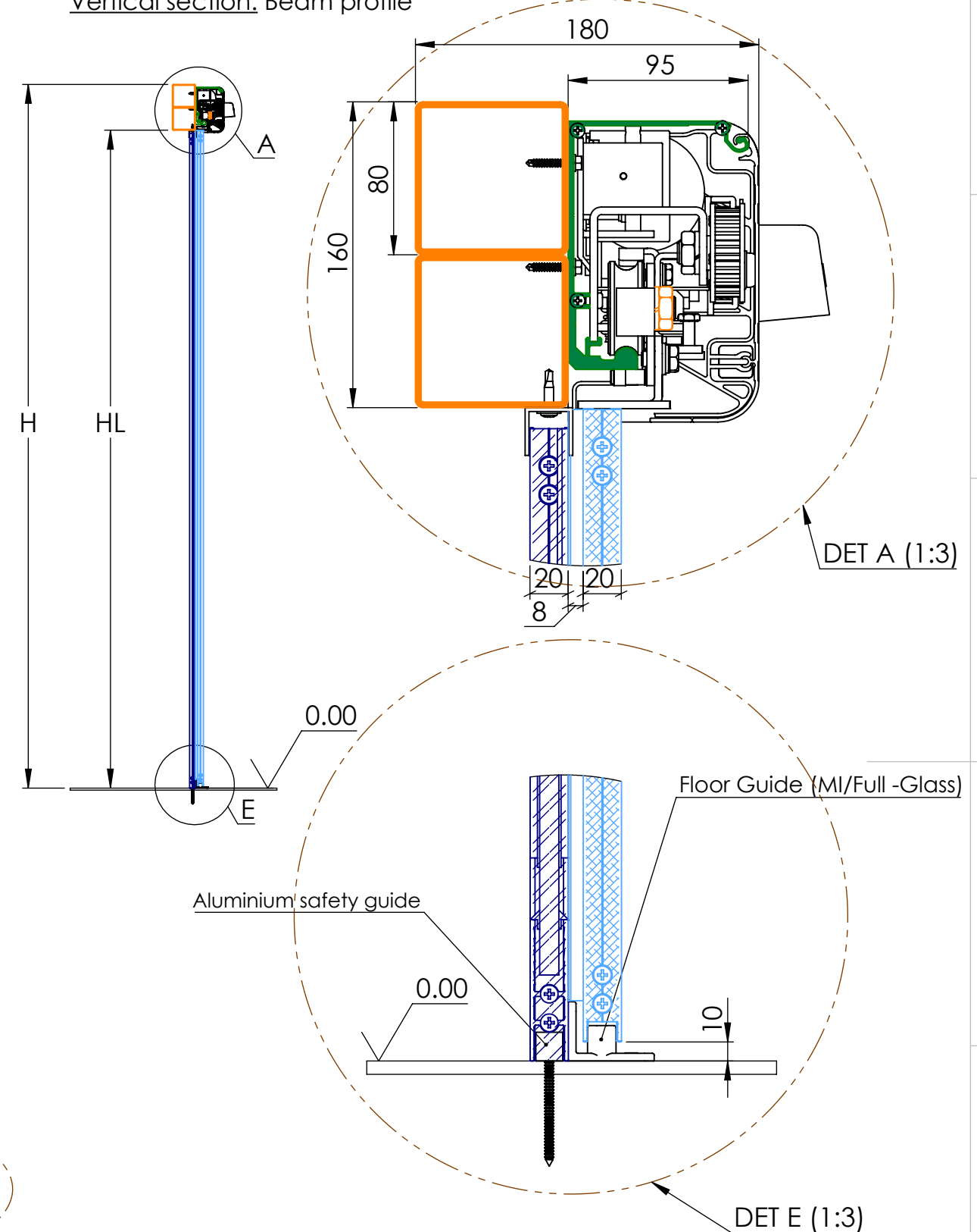
Vertical section: Beam profile
